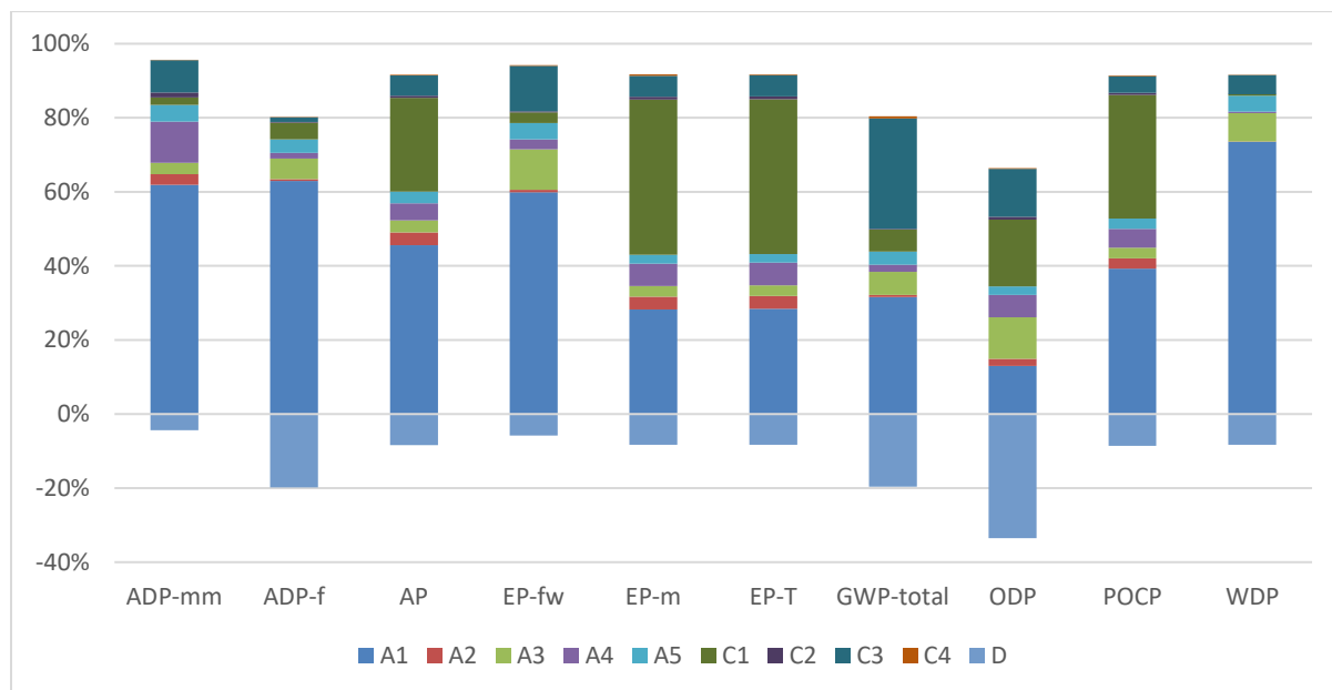
Figure 2: Tensar® TriAx® TX160 - Impact of the individual modules on the environmental core indicators (NMD set 2)
