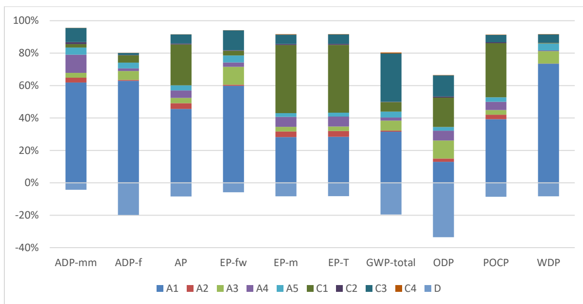
Figure 2: Tensar® TriAx® TX130S - Impact of the individual modules on the environmental core indicators (NMD set 2)
